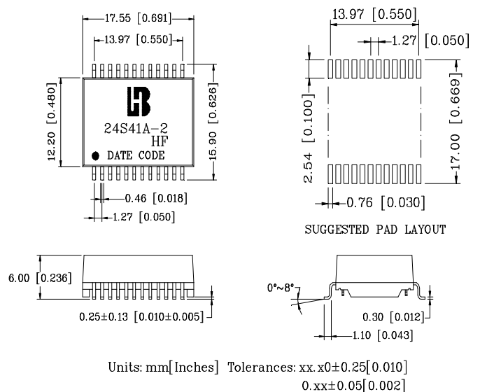
24HST Series Semi-open frame Type
