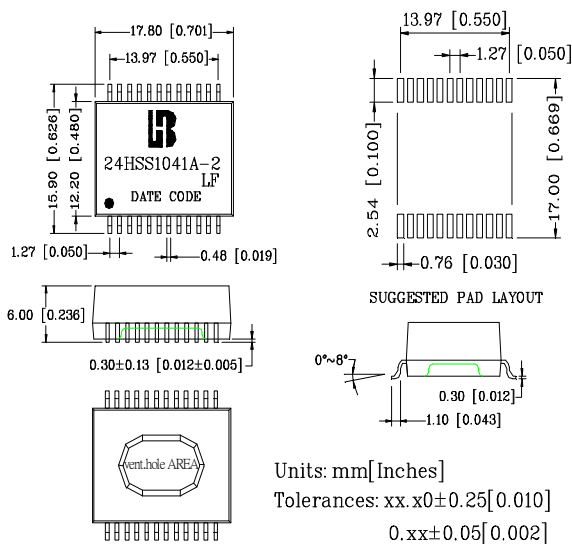
24HST Series Molding Type
